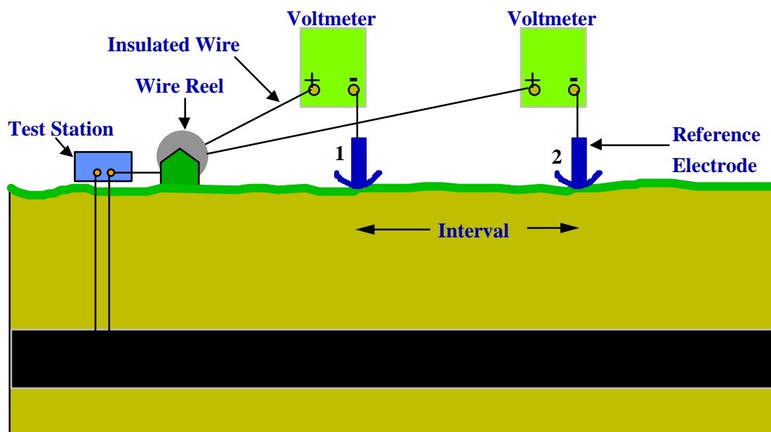
Figure 6 Single Electrode Potential Survey
